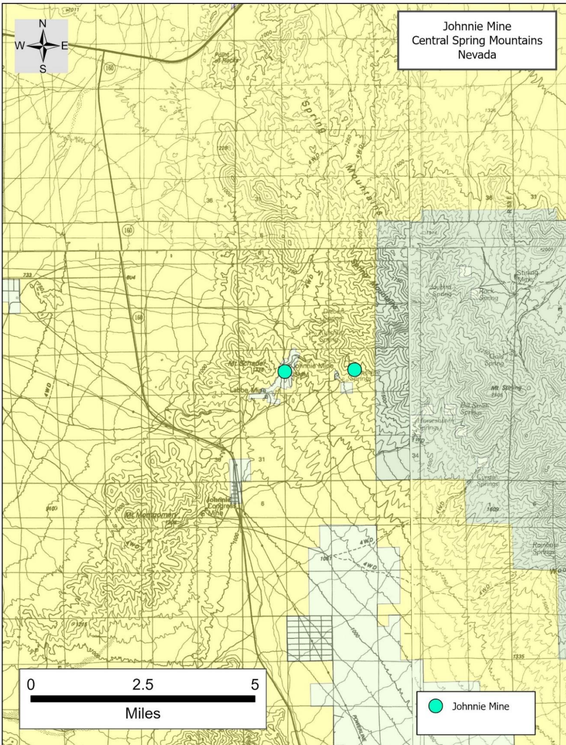
Figure 16. Land status map of the Johnnie District and surrounding areas. Green is U.S. Forest Service. Yellow is U.S. Bureau of Land Management. Blue is private land. Purple is military lands. Open source for educational purposes. No copyright.
