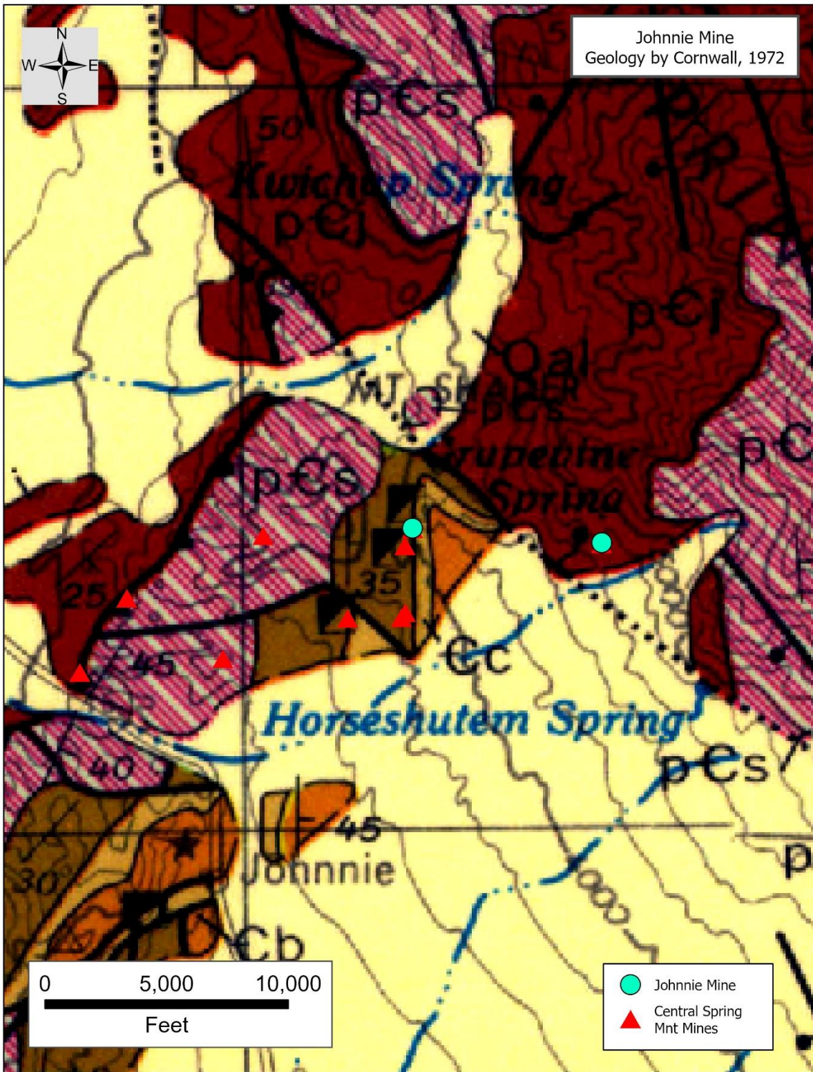
Figure 19. Regional geologic map of the area surrounding the Johnnie Mine. Open source for educational purposes. No copyright.
