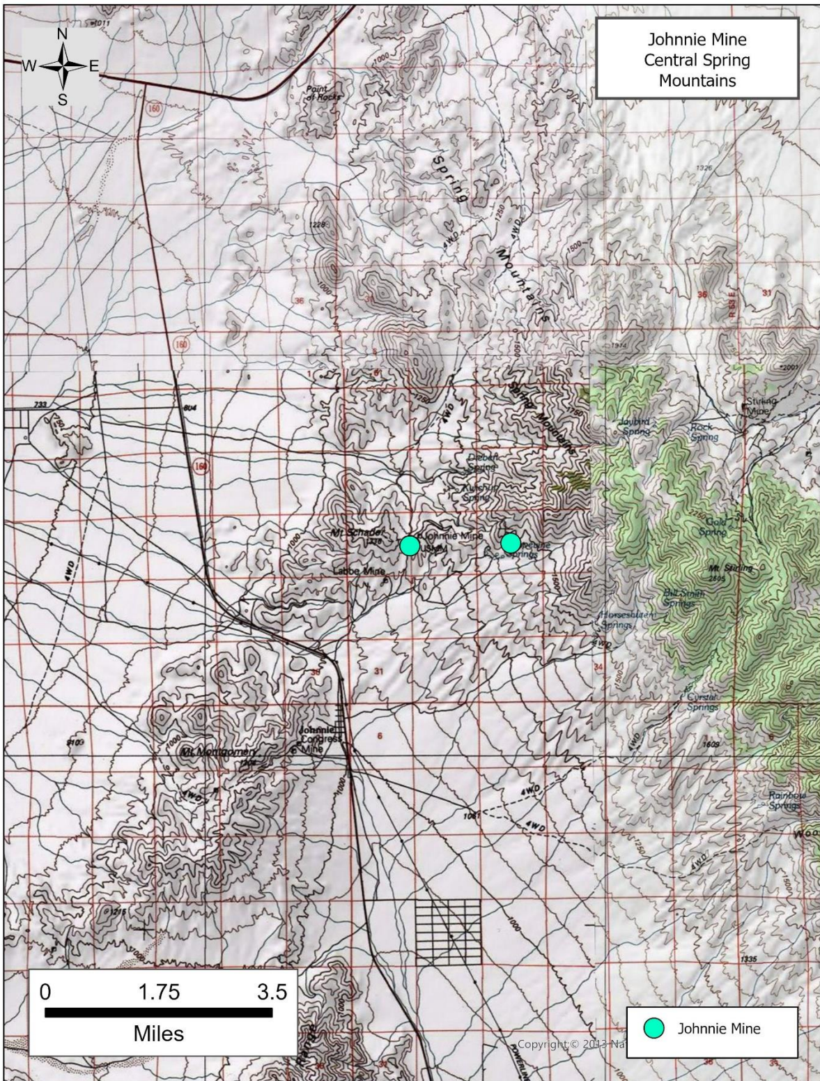
Figure 15. Regional topographic map of the Johnnie Mine. Open source for educational purposes. No copyright.
