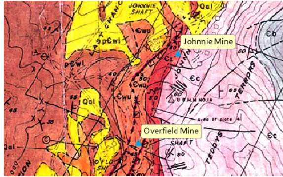
Figure 4. Portion of geologic map by Ivosevic, 1976. Open source for educational purposes. No copyright.
