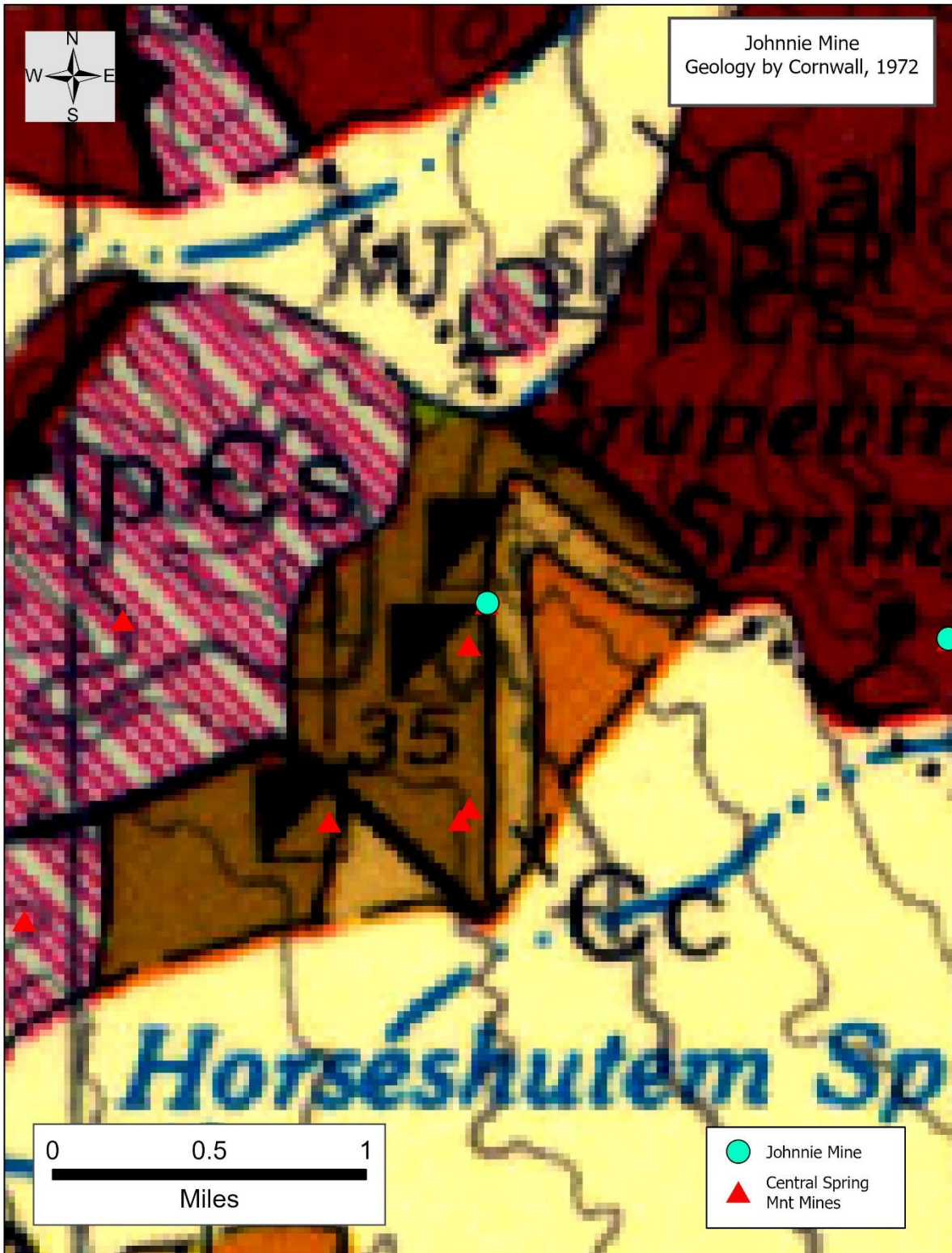
Figure 22. Area geologic map of the Johnnie Mine. Open source for educational purposes. No copyright.
