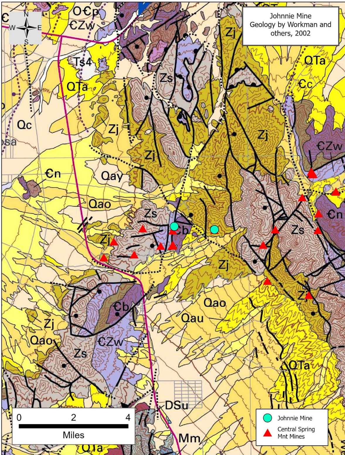
Figure 18. Regional geologic map of the area surrounding the Johnnie Mine. Open source for educational purposes. No copyright.
