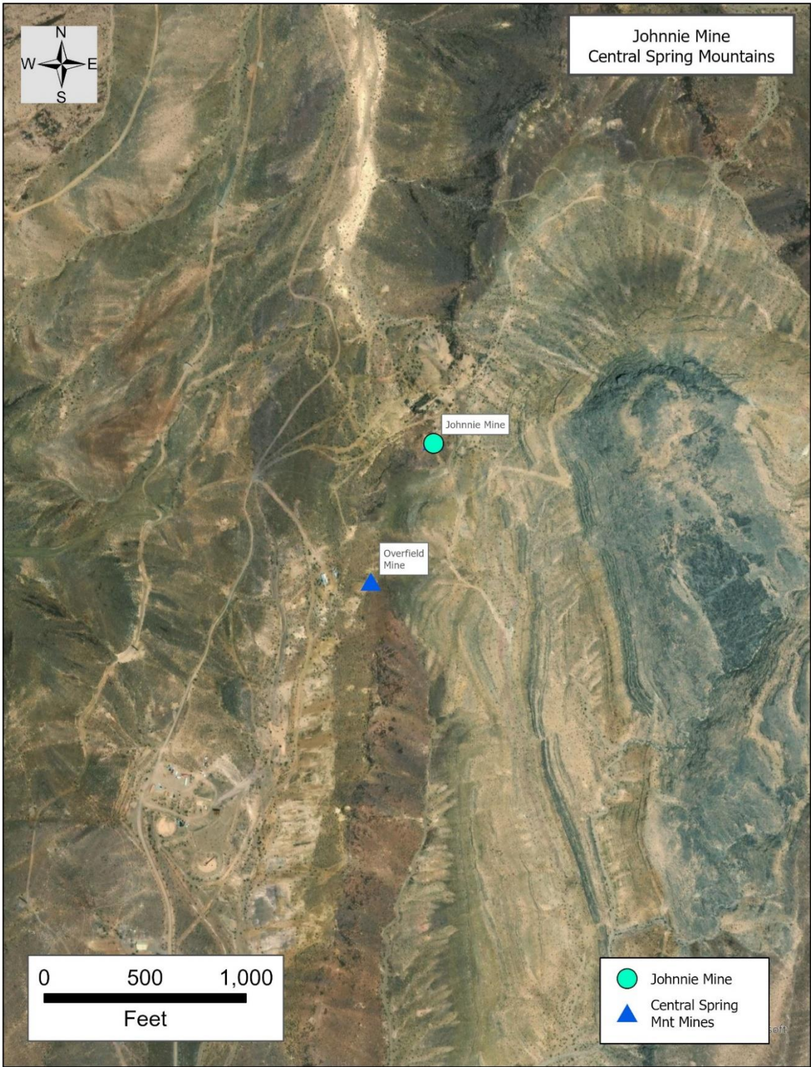
Figure 25. Aerial photograph of the Johnnie Mine. Open source for educational purposes. No copyright.
