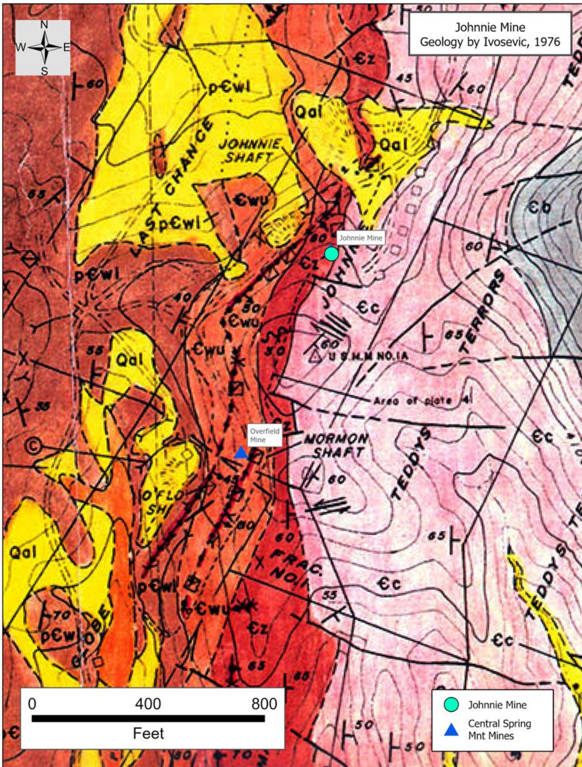
Figure 26. Site geologic map of the Johnnie mine and surrounding areas. Open source for educational purposes. No copyright.
