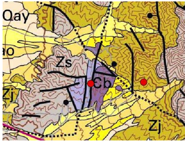
Figure 2. Portion of geologic map by Workman and others, 2022. Open source for educational purposes. No copyright.
