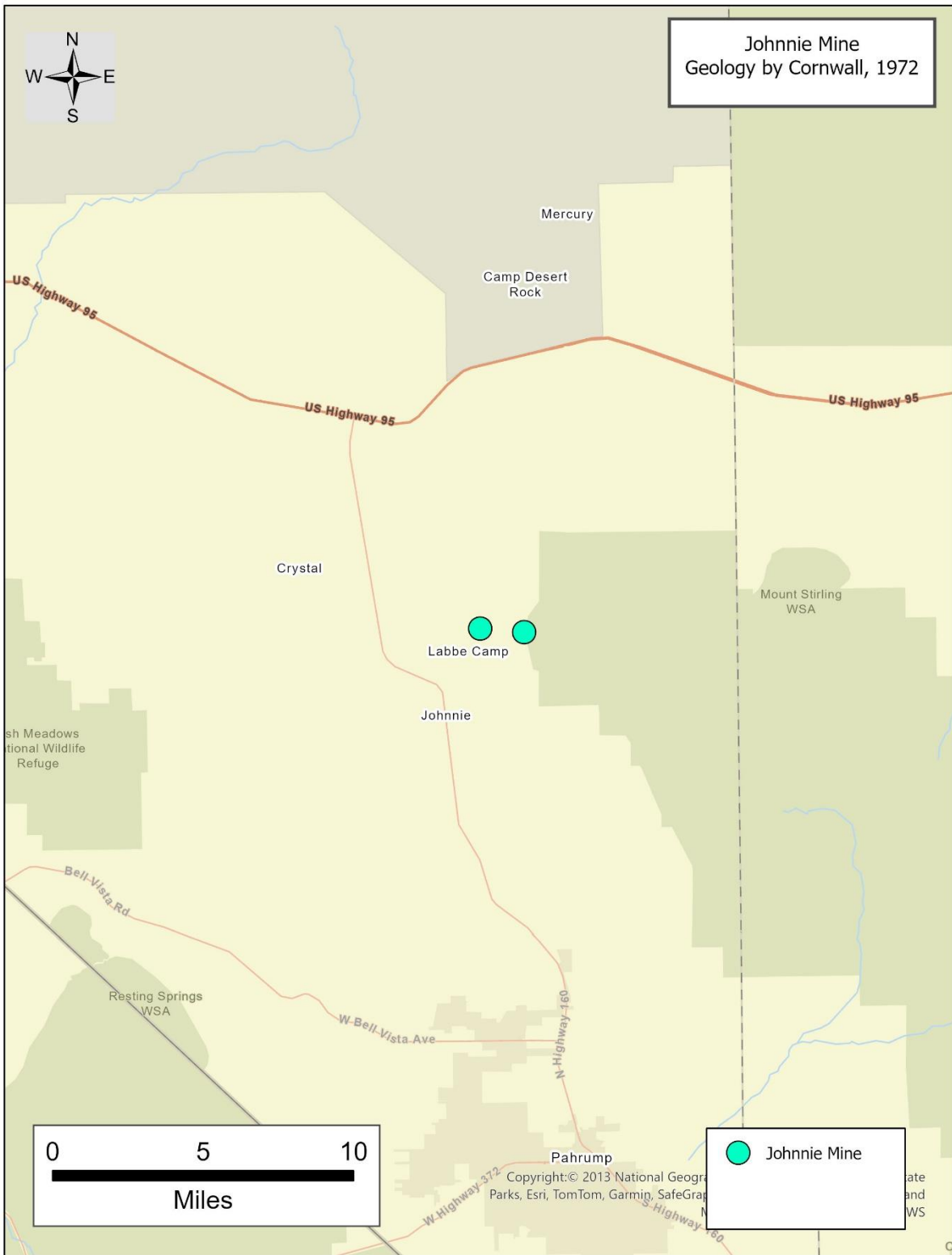
Figure 14. Location map for the Johnnie Mine. Open source for educational purposes. No copyright.
