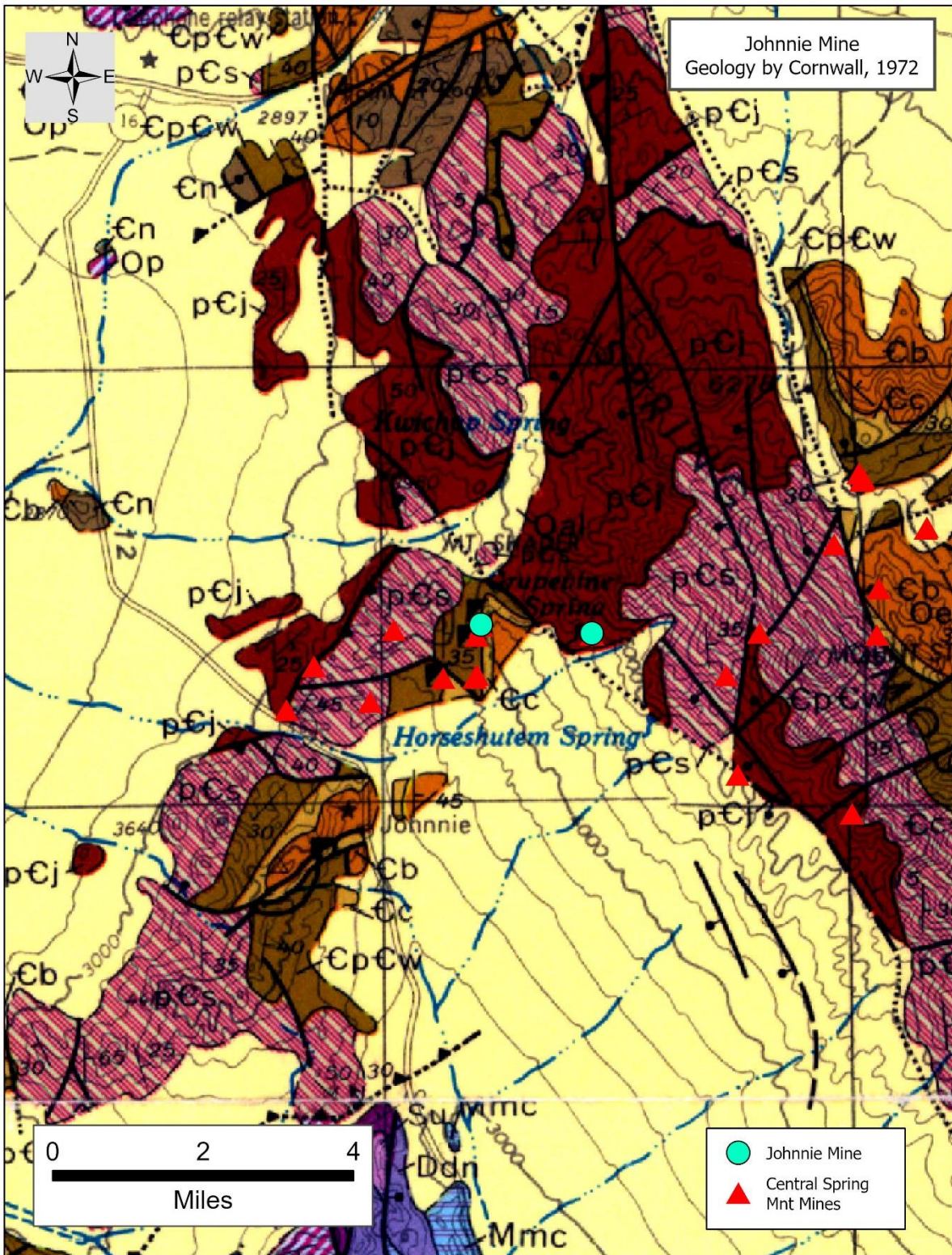
Figure 17. Regional geologic map of the Johnnie mine and surrounding areas. Open source for educational purposes. No copyright.
